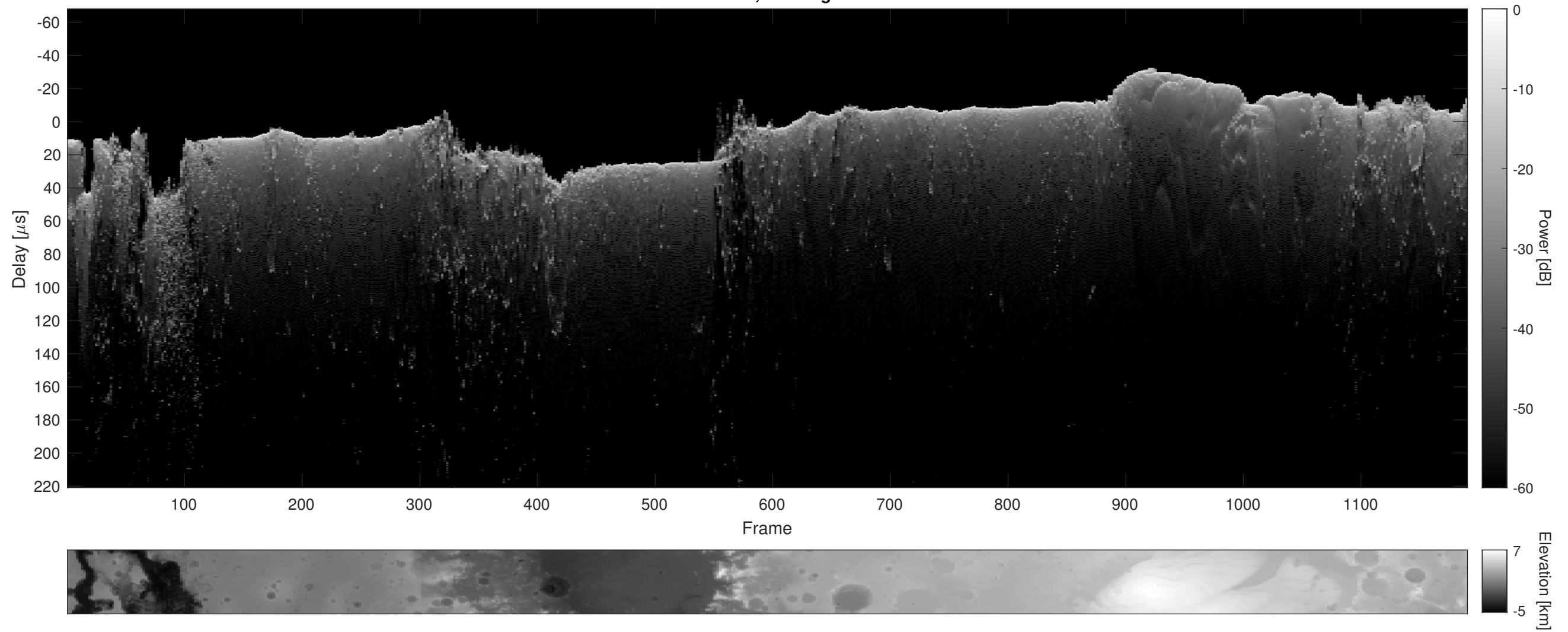
Orbit 8918, Cluttergram
