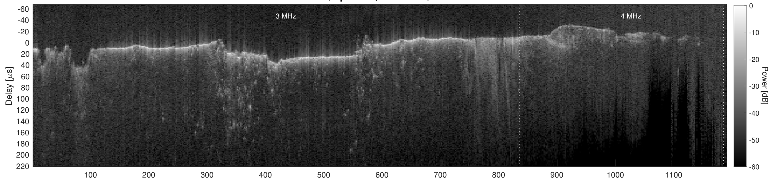
Orbit 8918, Cluttergram
