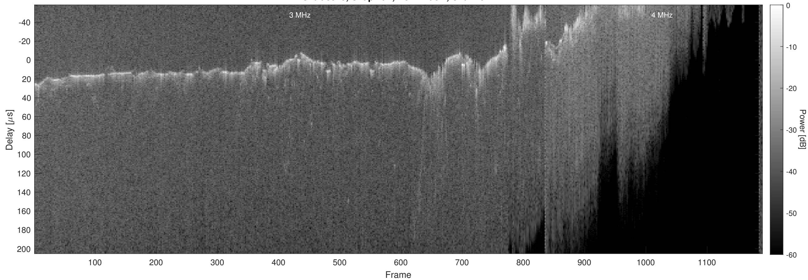
Orbit 8919, Chapman, No Window, Channel 2
