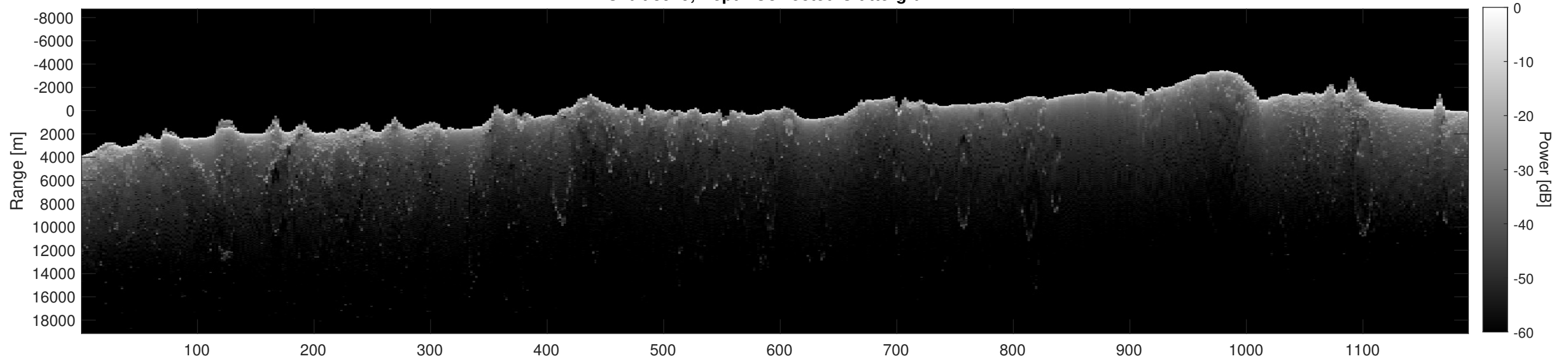
Orbit 8919, Depth-Corrected Cluttergram
