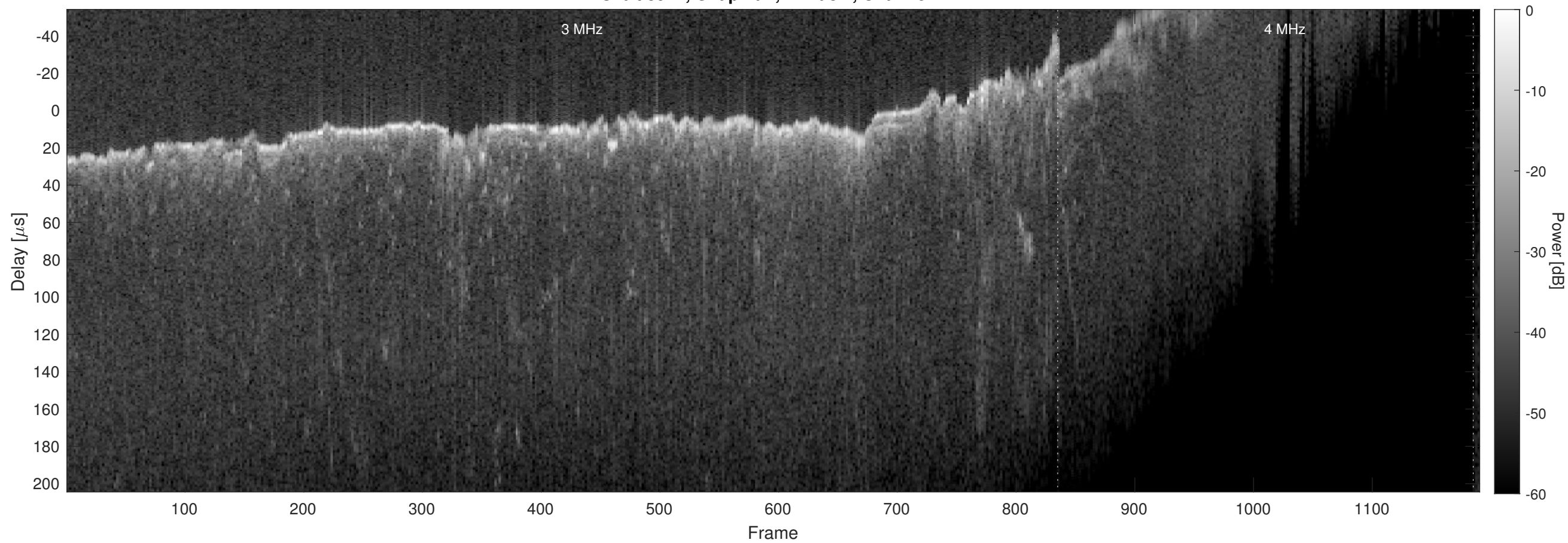
Orbit 8921, Chapman, Window, Channel 2
