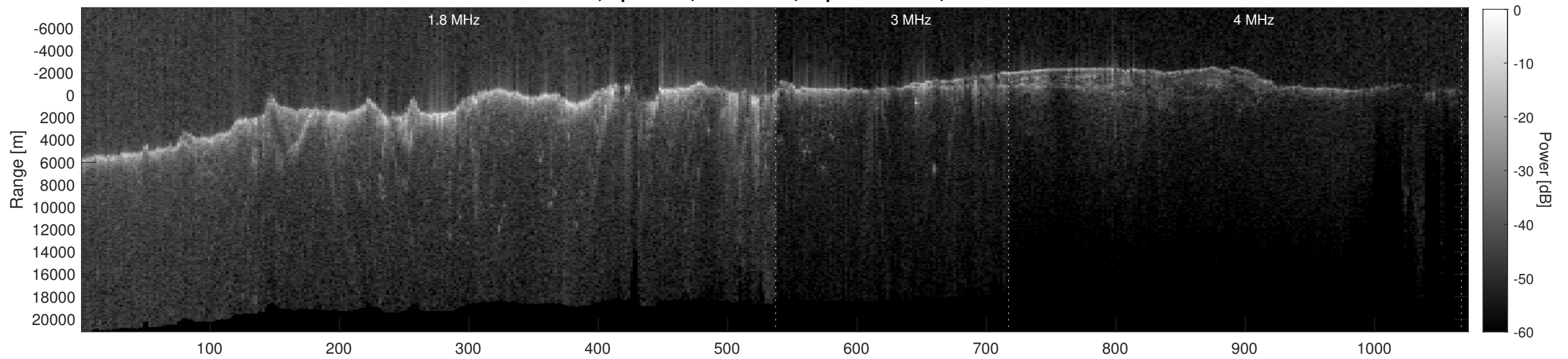
Orbit 8923, Depth-Corrected Cluttergram
