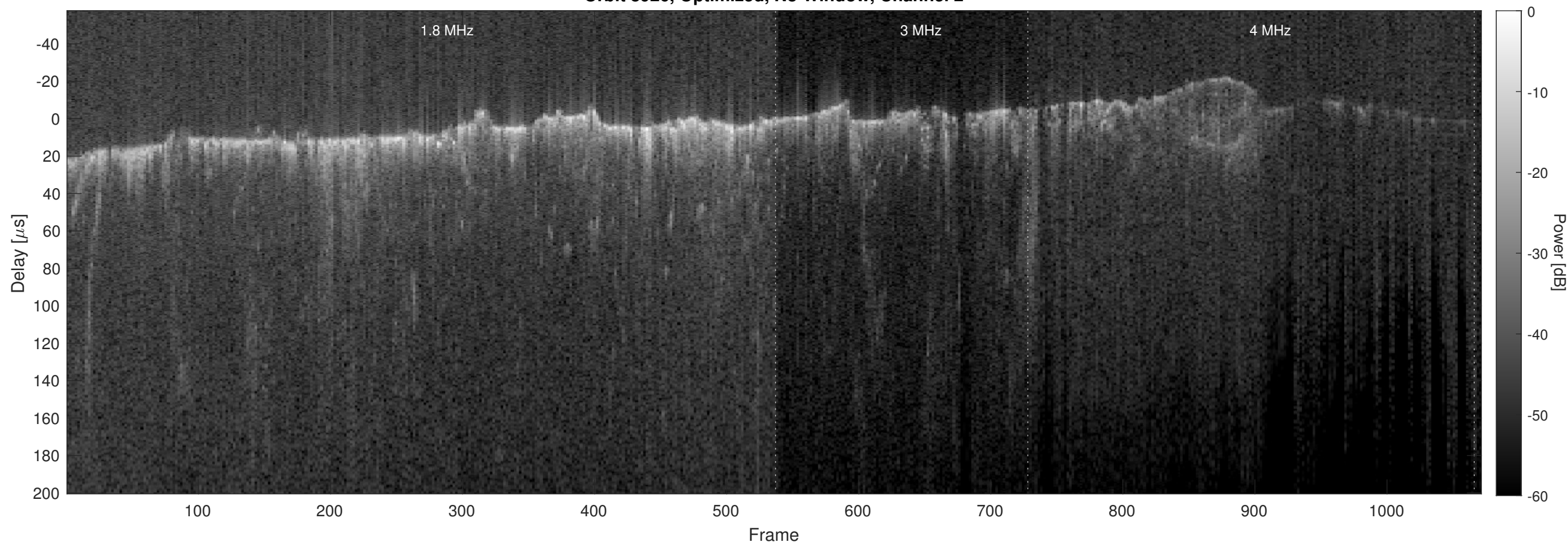
Orbit 8926, Optimized, No Window, Channel 2
