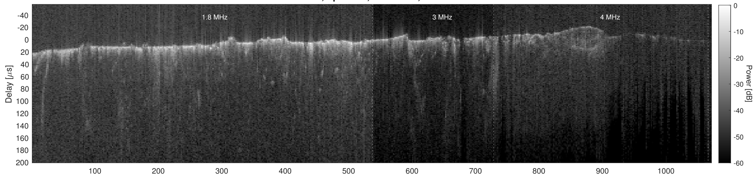
Orbit 8926, Cluttergram
