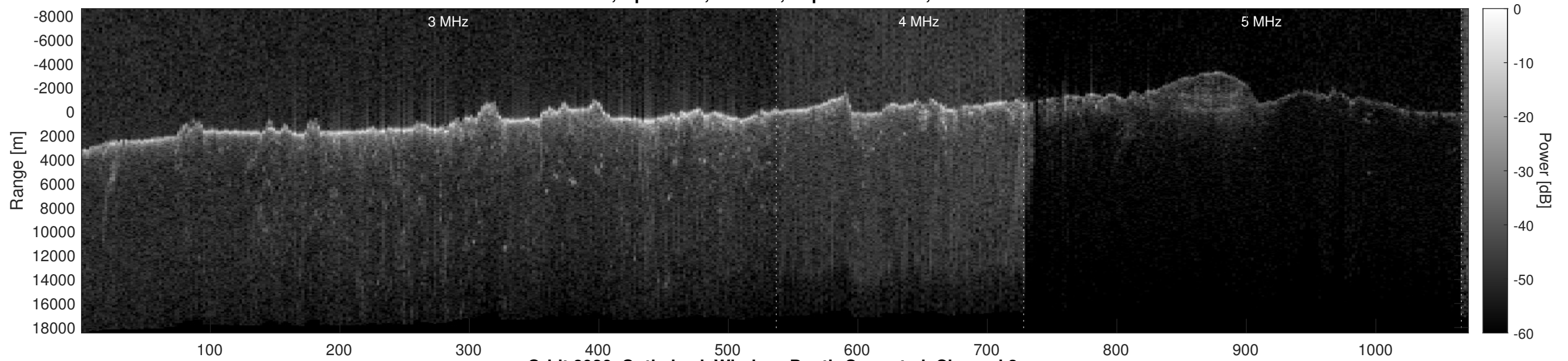
Orbit 8926, Optimized, Window, Depth-Corrected, Channel 2
