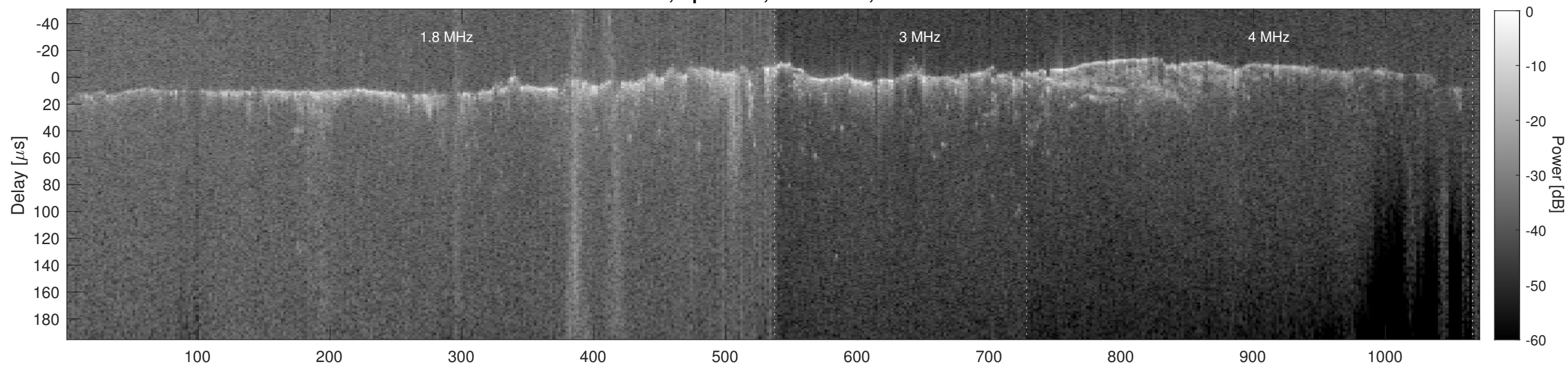
Orbit 8927, Cluttergram
