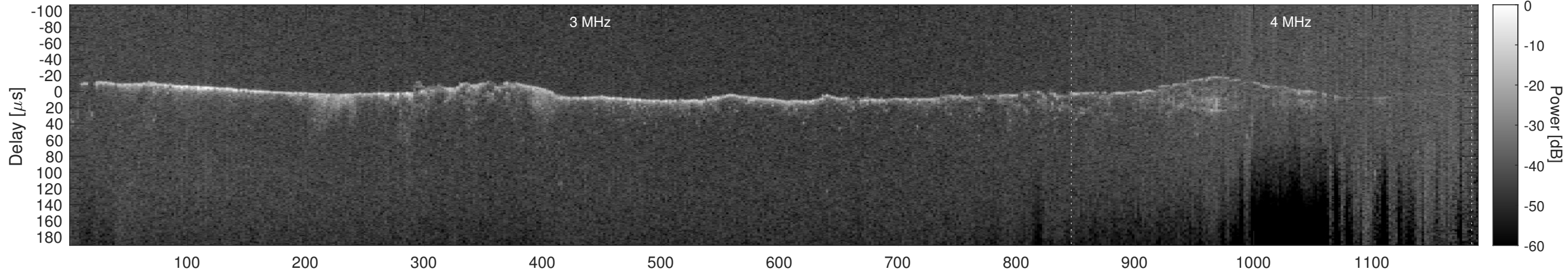
Orbit 8929, Cluttergram
