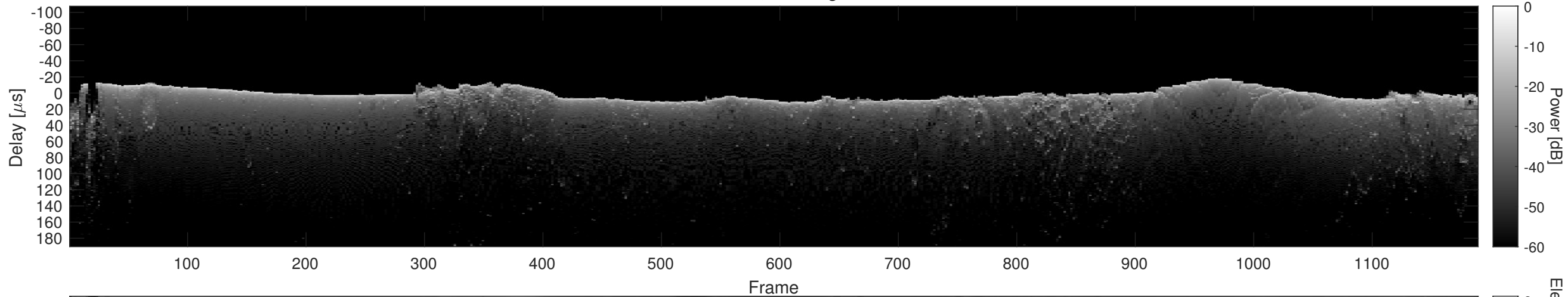
Orbit 8929, Cluttergram
