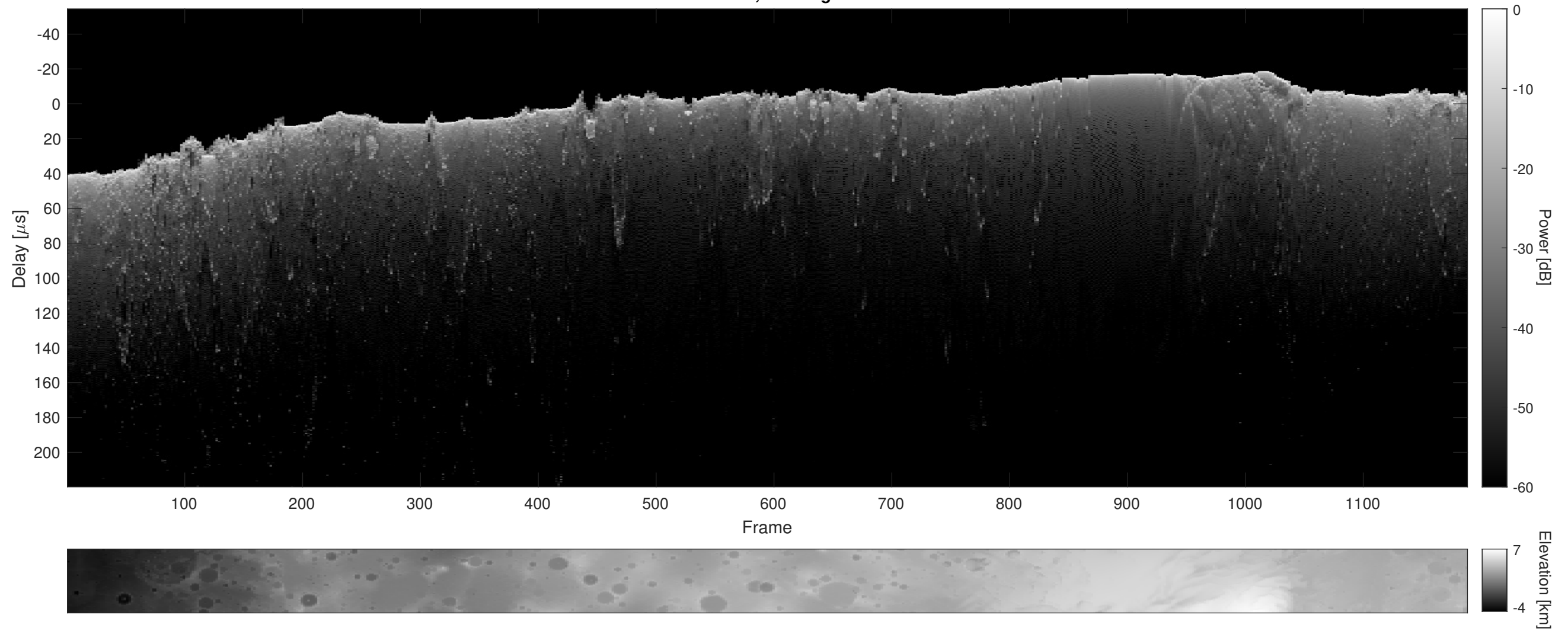
Orbit 8930, Cluttergram
