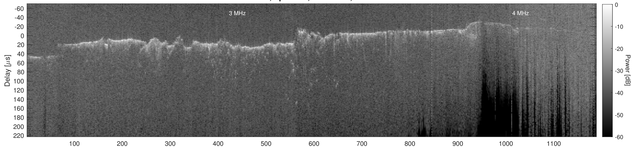
Orbit 8932, Cluttergram
