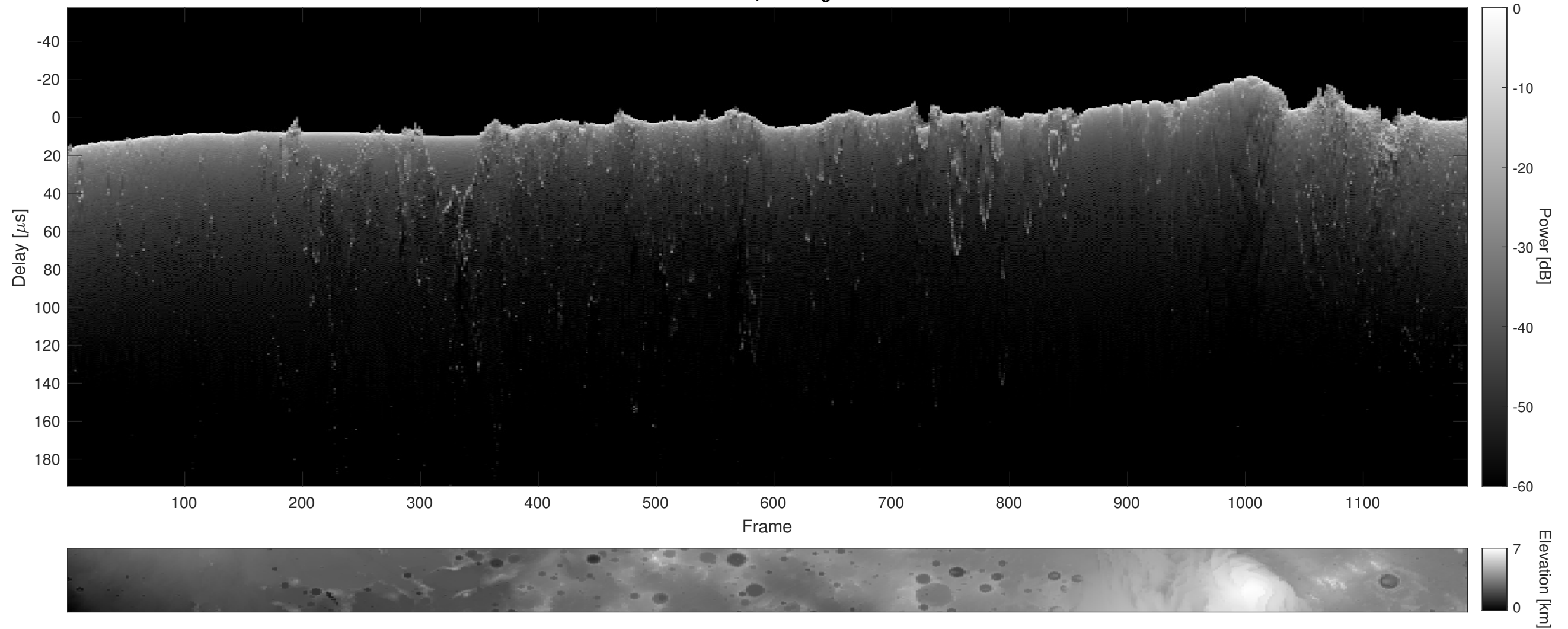
Orbit 8933, Cluttergram
