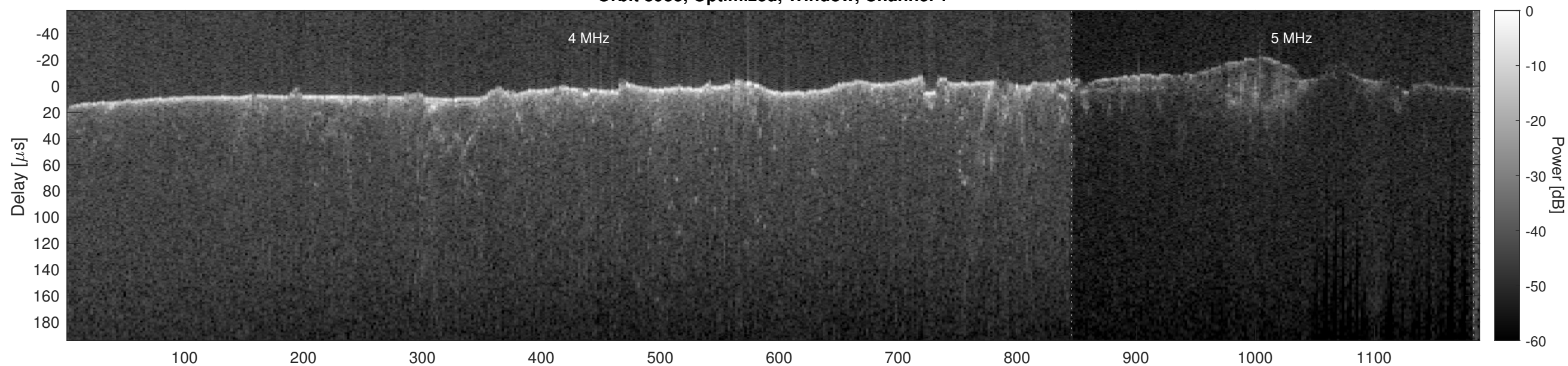
Orbit 8933, Optimized, Window, Channel 2
