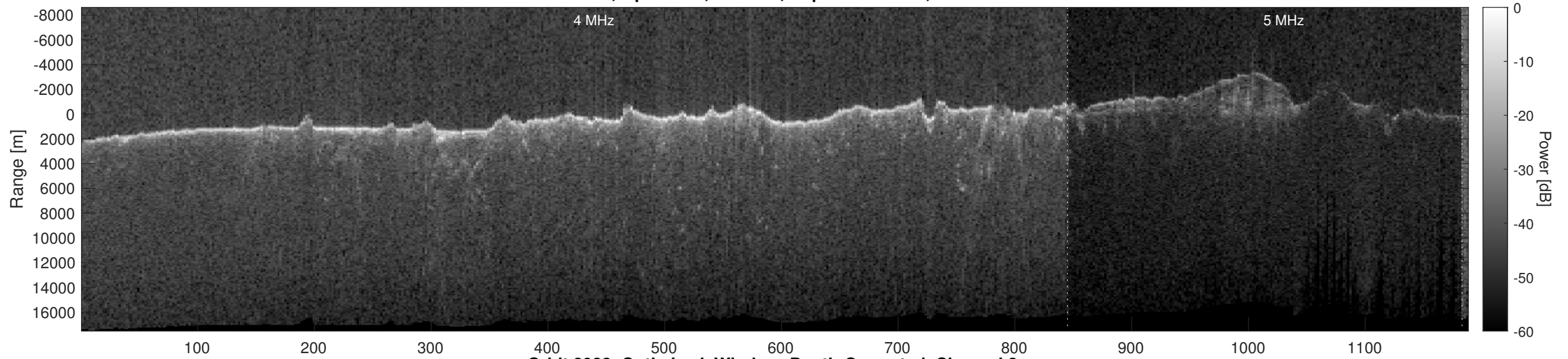
Orbit 8933, Optimized, Window, Depth-Corrected, Channel 2
