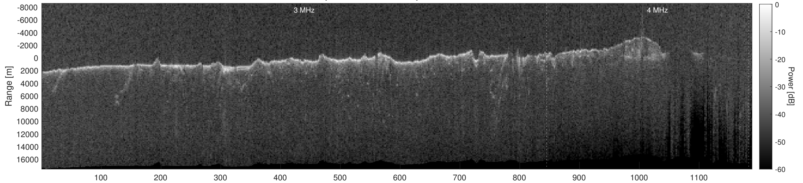
Orbit 8933, Depth-Corrected Cluttergram
