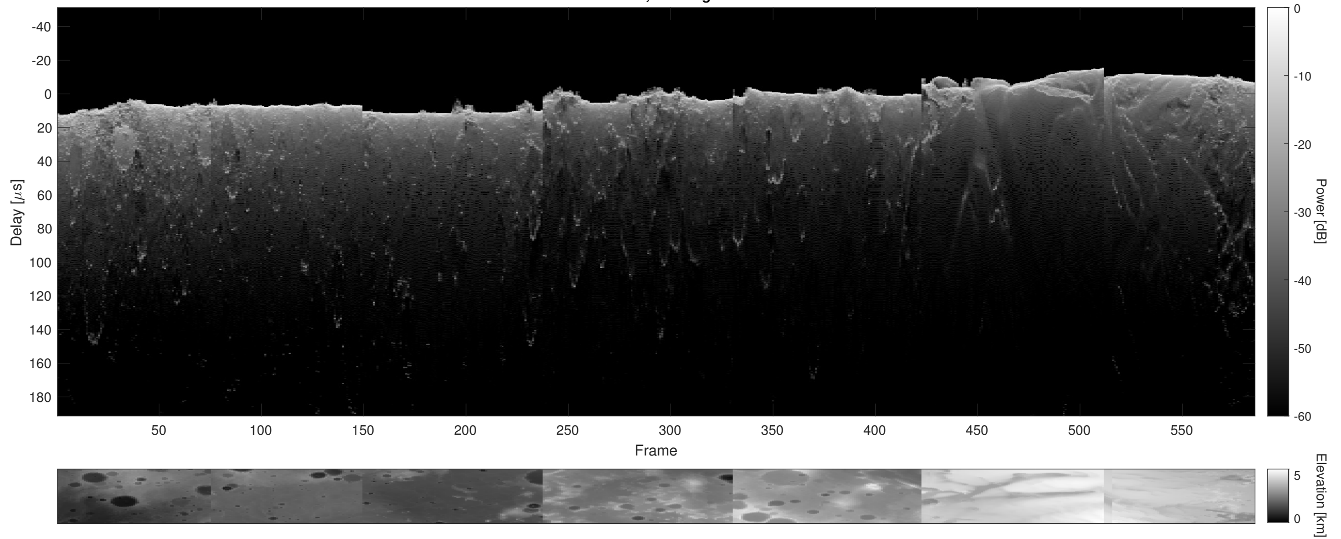
Orbit 8934, Cluttergram
