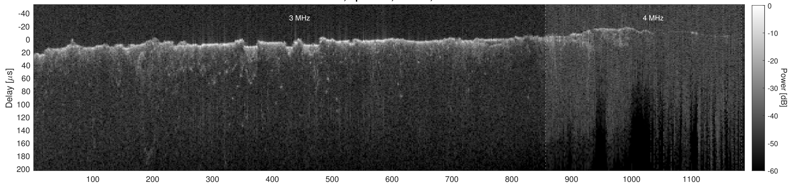
Orbit 8935, Cluttergram
