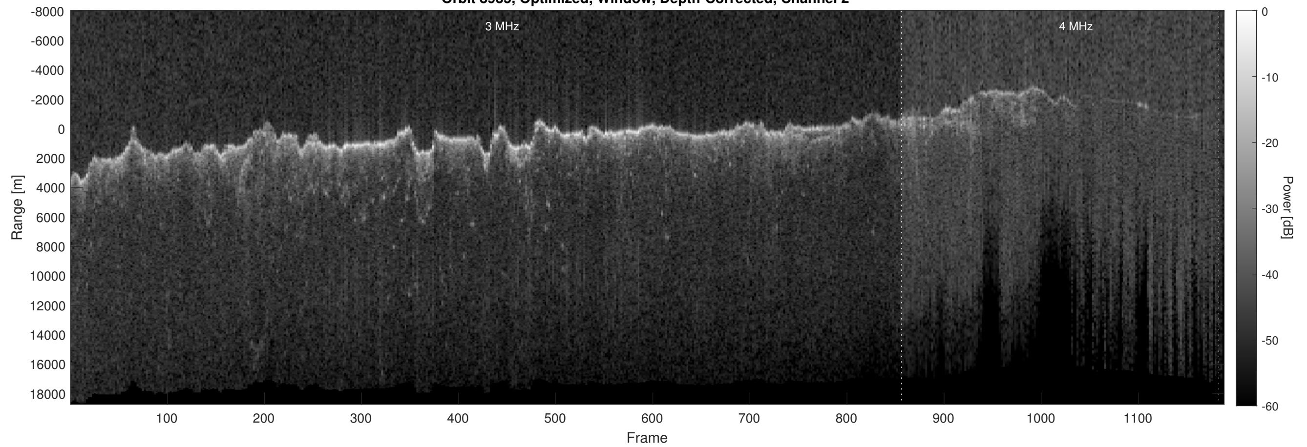
Orbit 8935, Optimized, Window, Depth-Corrected, Channel 2
