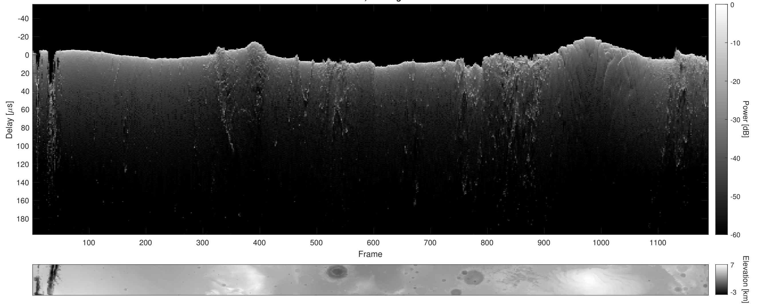
Orbit 8936, Cluttergram
