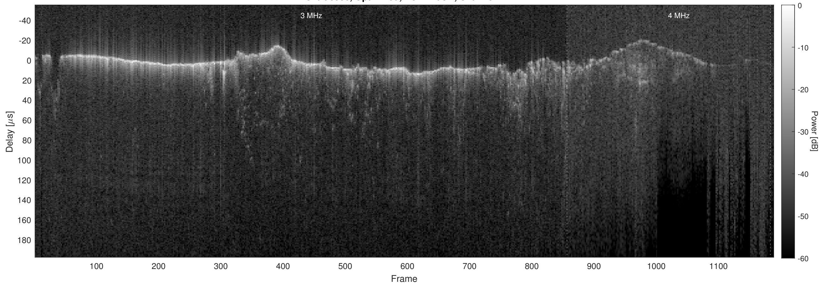
Orbit 8936, Optimized, No Window, Channel 2
