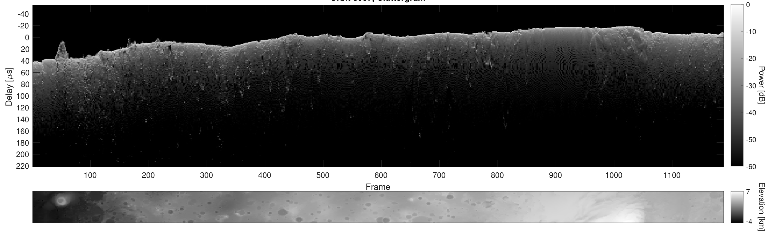
Orbit 8937, Cluttergram
