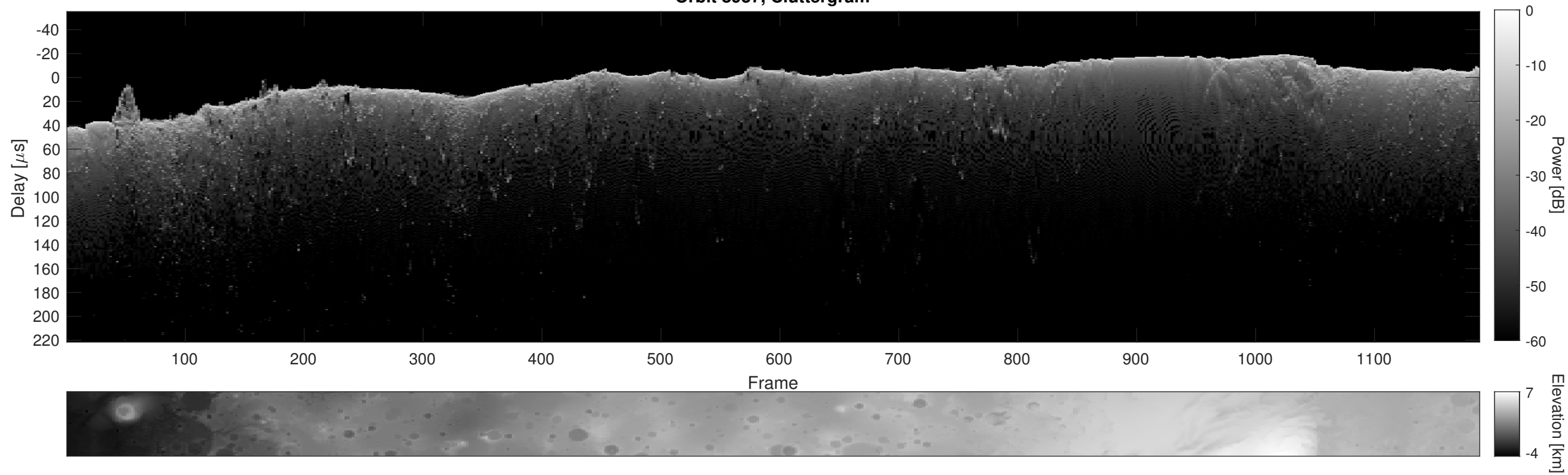
Orbit 8937, Cluttergram
