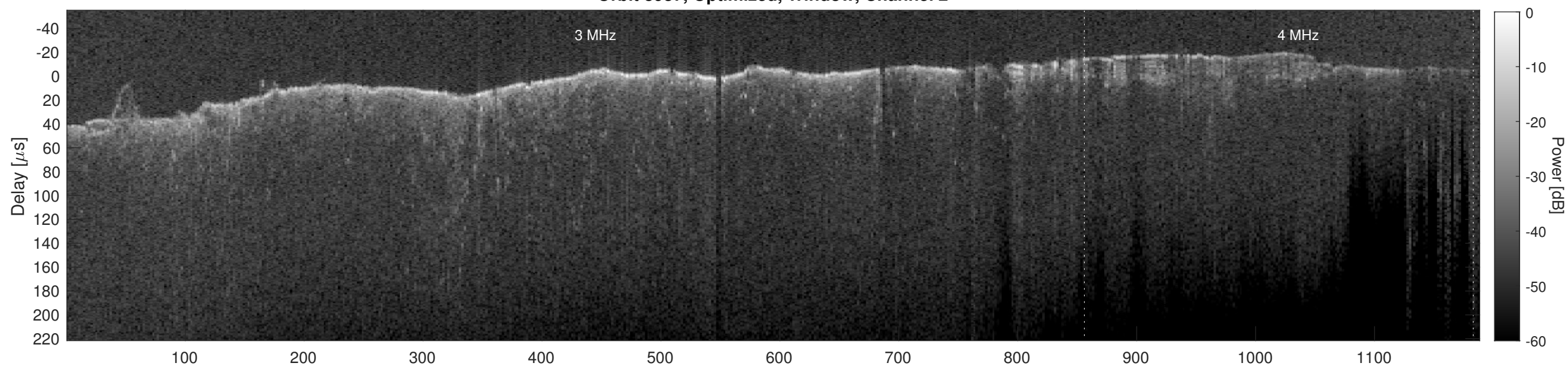
Orbit 8937, Cluttergram
