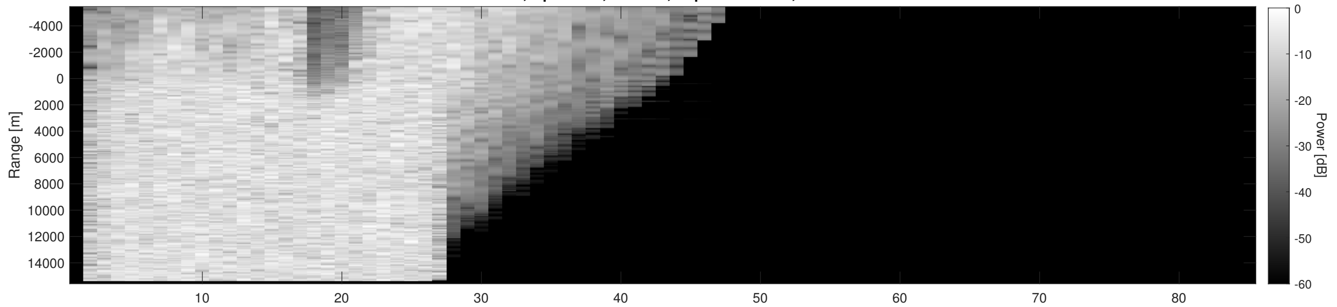
Orbit 8939, Depth-Corrected Cluttergram
