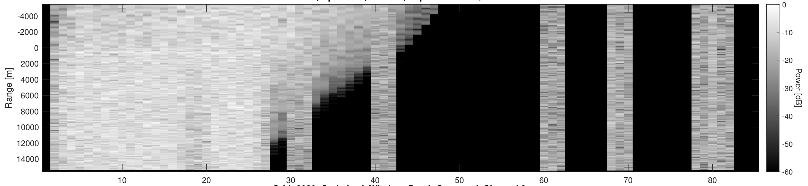
Orbit 8939, Optimized, Window, Depth-Corrected, Channel 2
