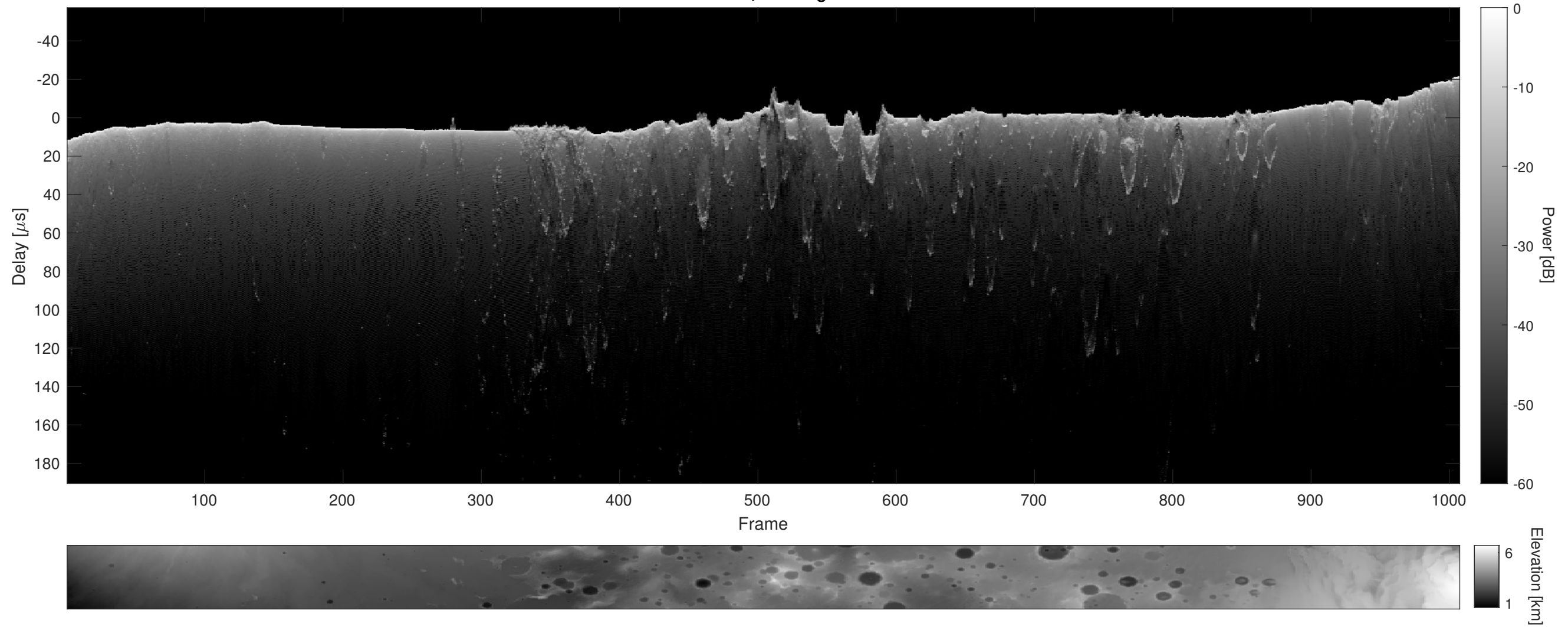
Orbit 8940, Cluttergram
