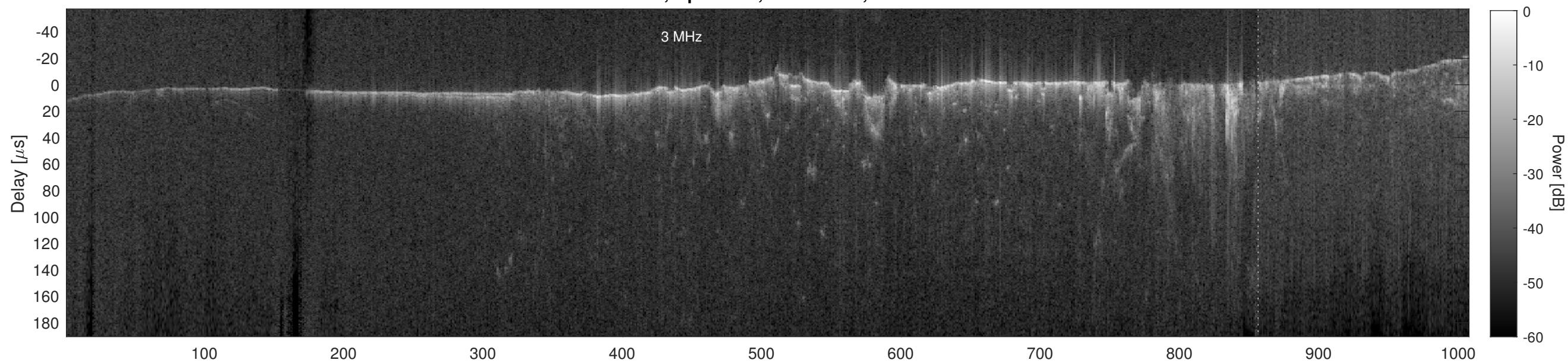
Orbit 8940, Cluttergram
