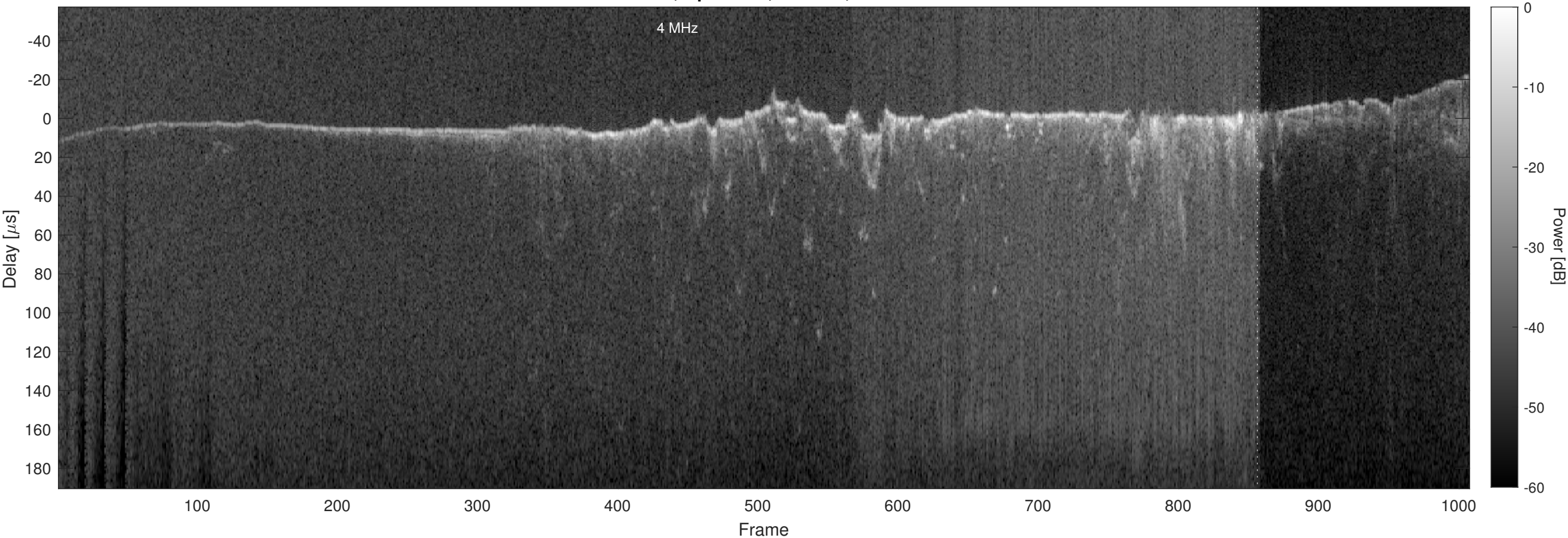
Orbit 8940, Optimized, Window, Channel 2
