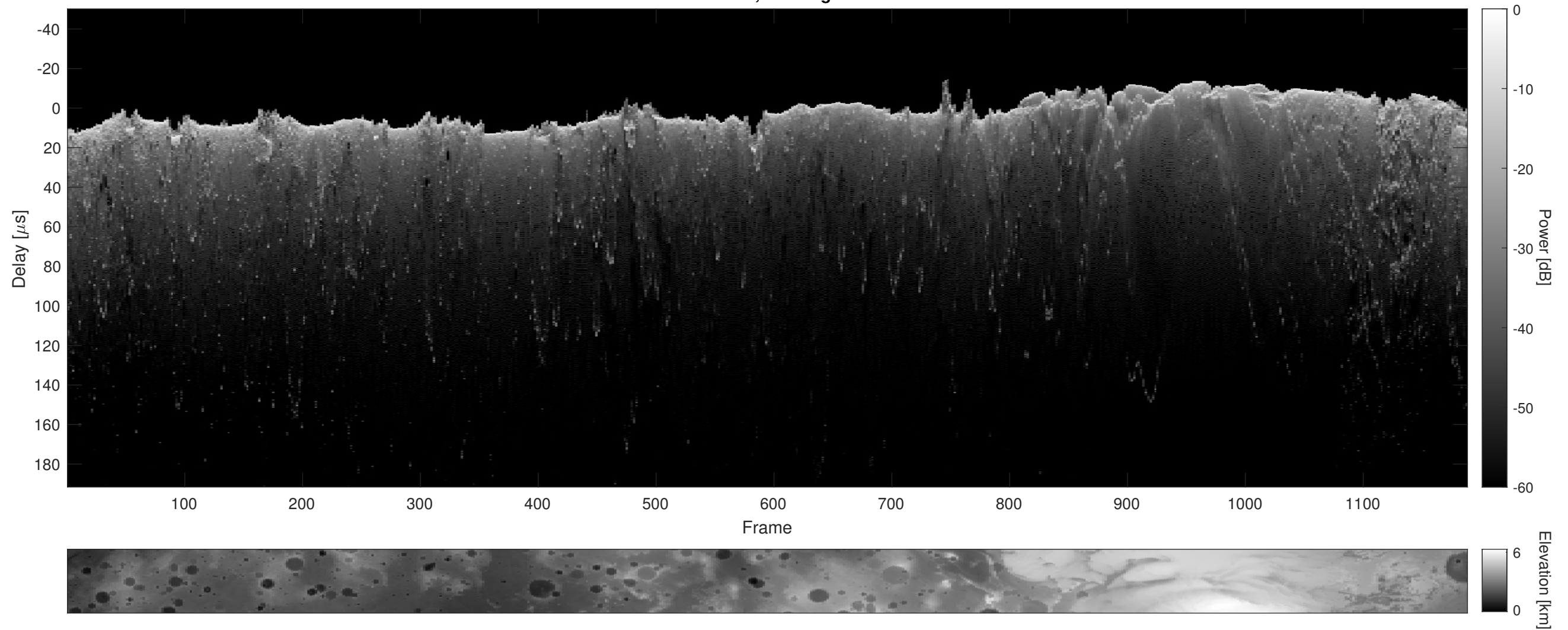
Orbit 8941, Cluttergram
