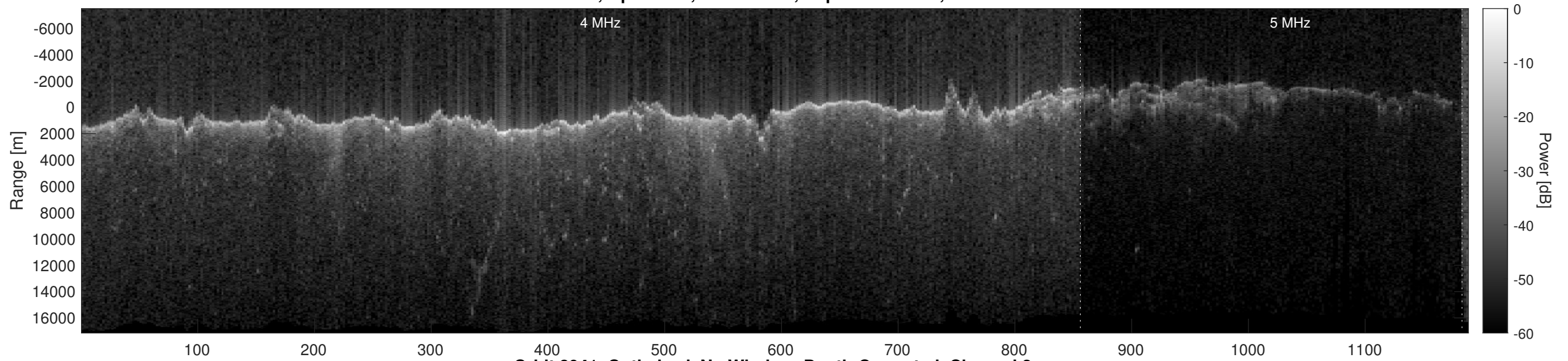
Orbit 8941, Optimized, No Window, Depth-Corrected, Channel 2
