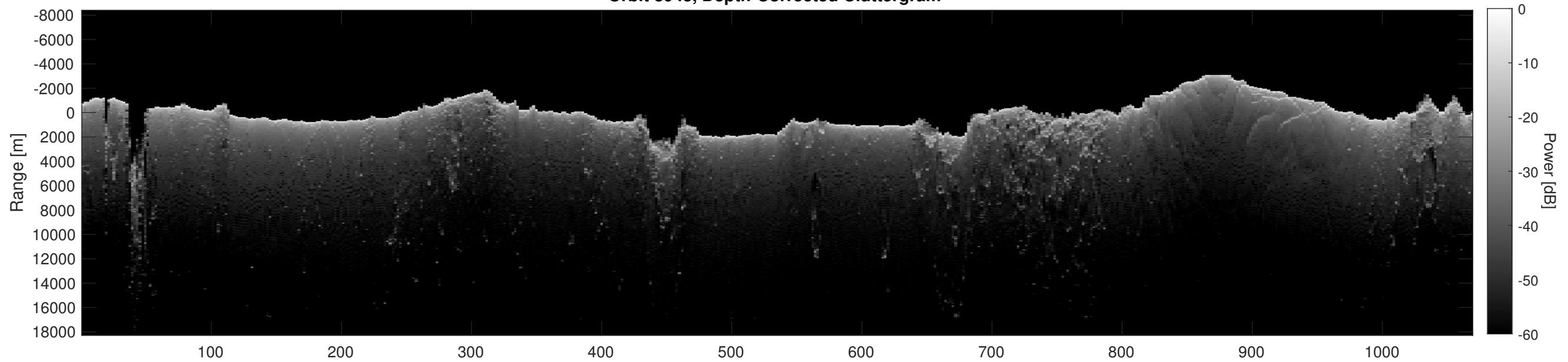
Orbit 8943, Depth-Corrected Cluttergram
