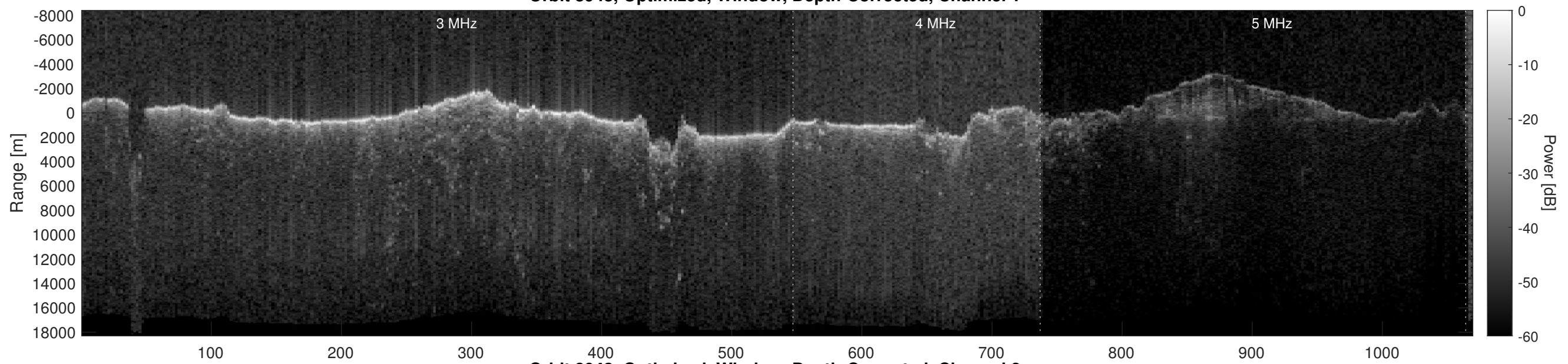
Orbit 8943, Optimized, Window, Depth-Corrected, Channel 2
