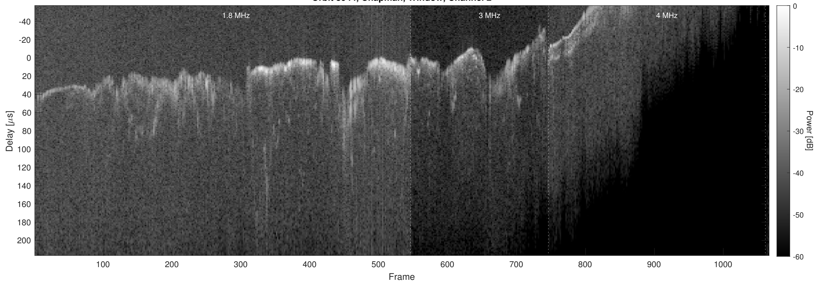
Orbit 8944, Chapman, Window, Channel 2
