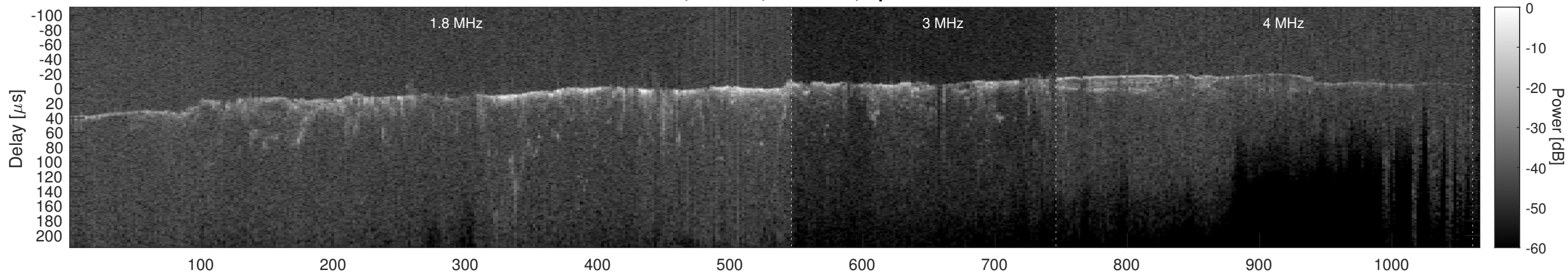
Orbit 8944, Cluttergram
