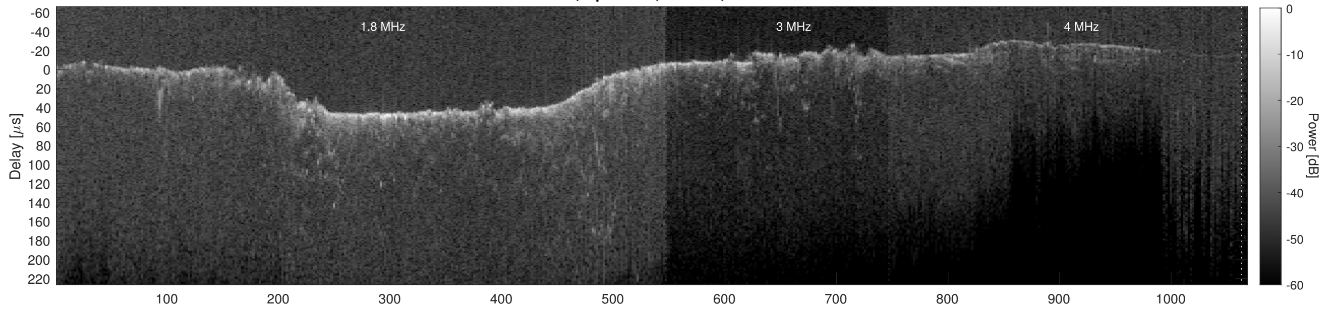
Orbit 8945, Cluttergram
