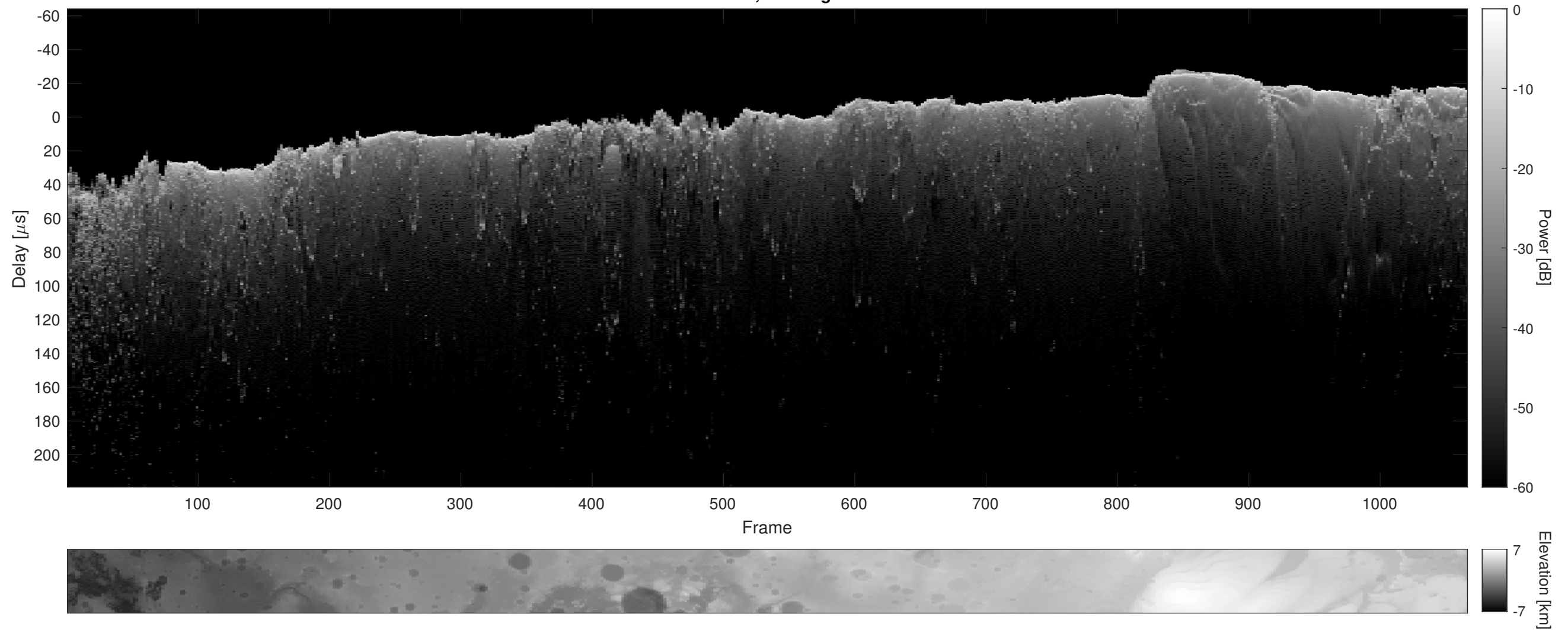
Orbit 8946, Cluttergram
