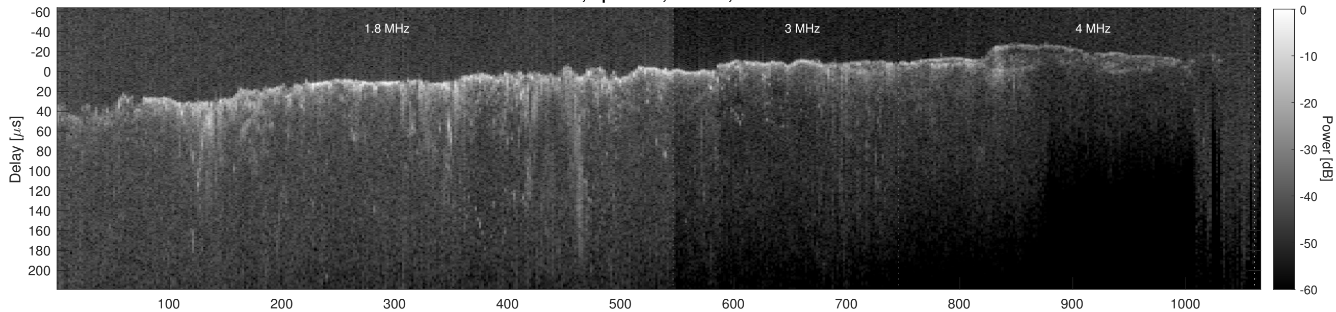
Orbit 8946, Cluttergram
