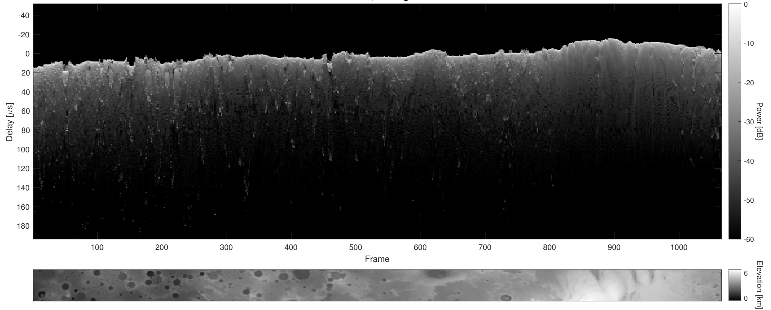
Orbit 8949, Cluttergram
