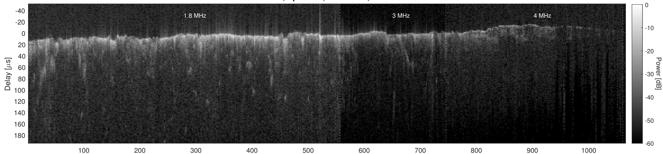
Orbit 8949, Cluttergram
