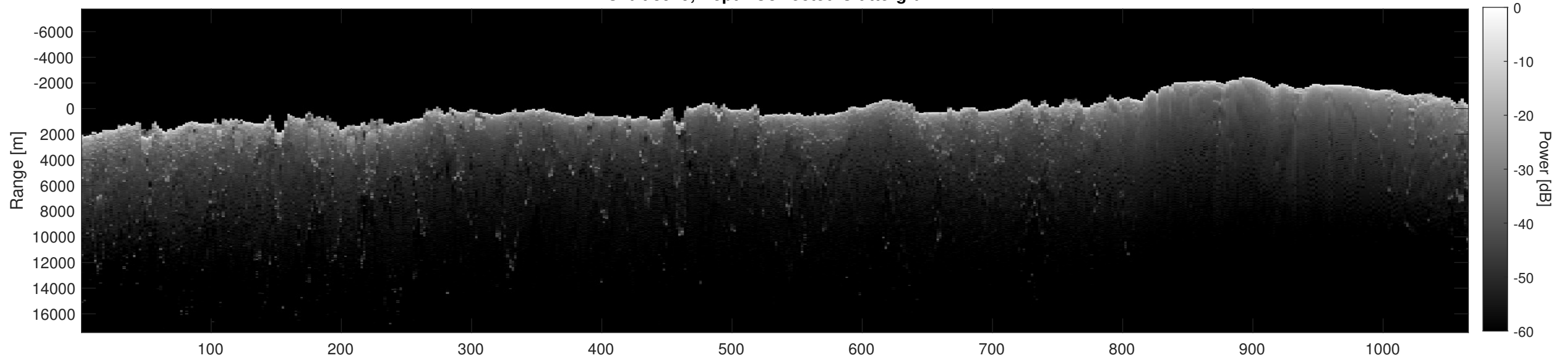
Orbit 8949, Depth-Corrected Cluttergram
