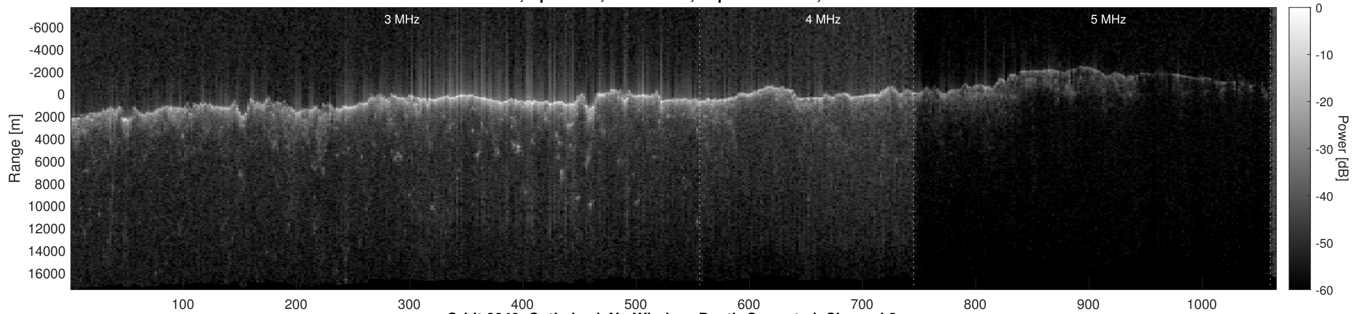
Orbit 8949, Optimized, No Window, Depth-Corrected, Channel 2
