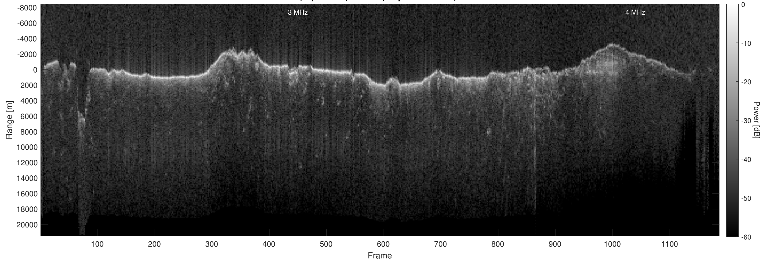
Orbit 8950, Optimized, Window, Depth-Corrected, Channel 2
