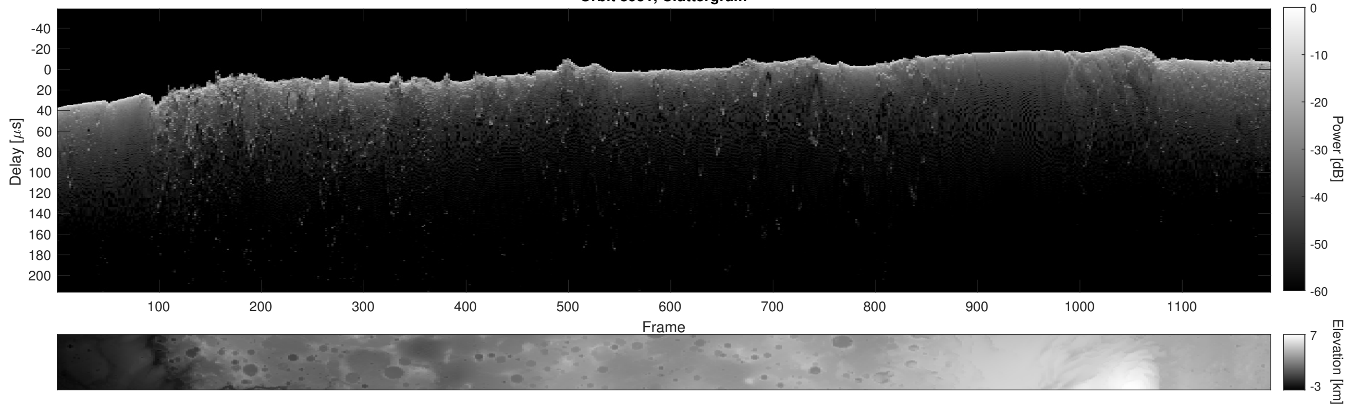
Orbit 8951, Cluttergram
