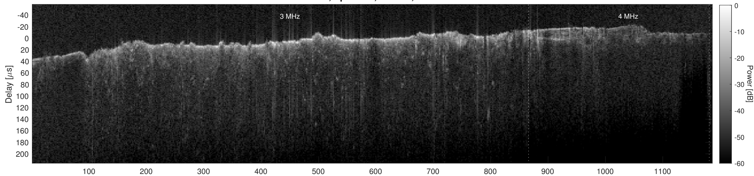
Orbit 8951, Cluttergram
