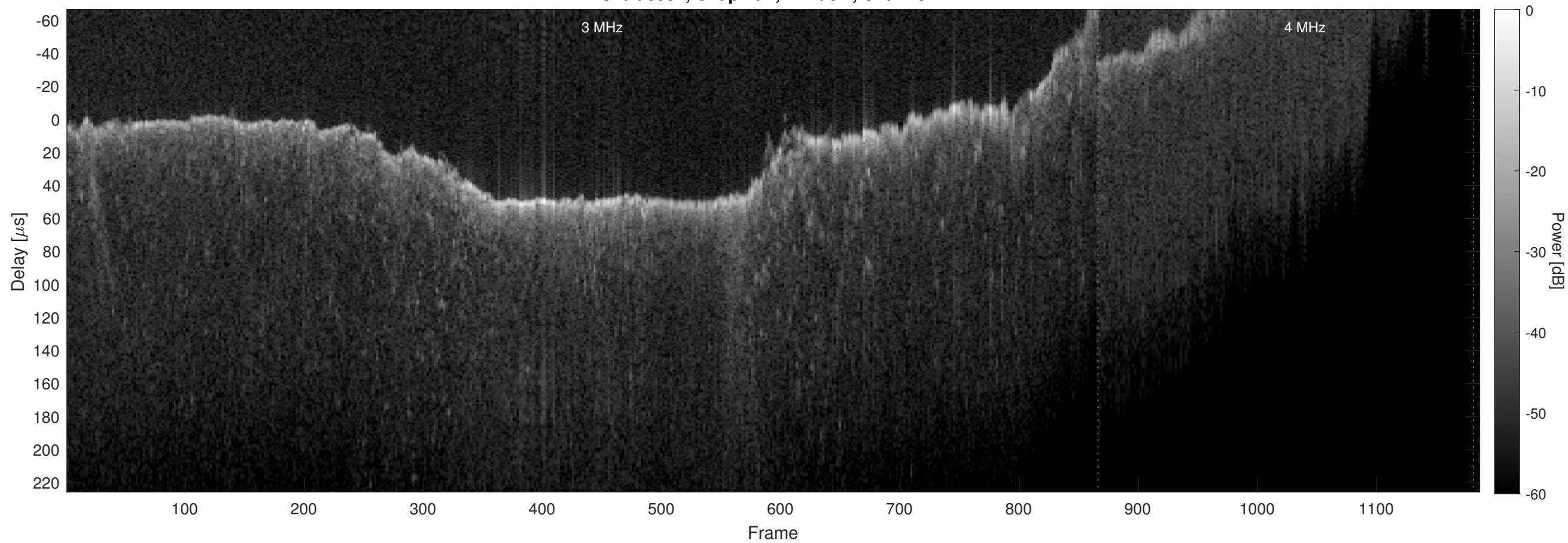
Orbit 8952, Chapman, Window, Channel 2
