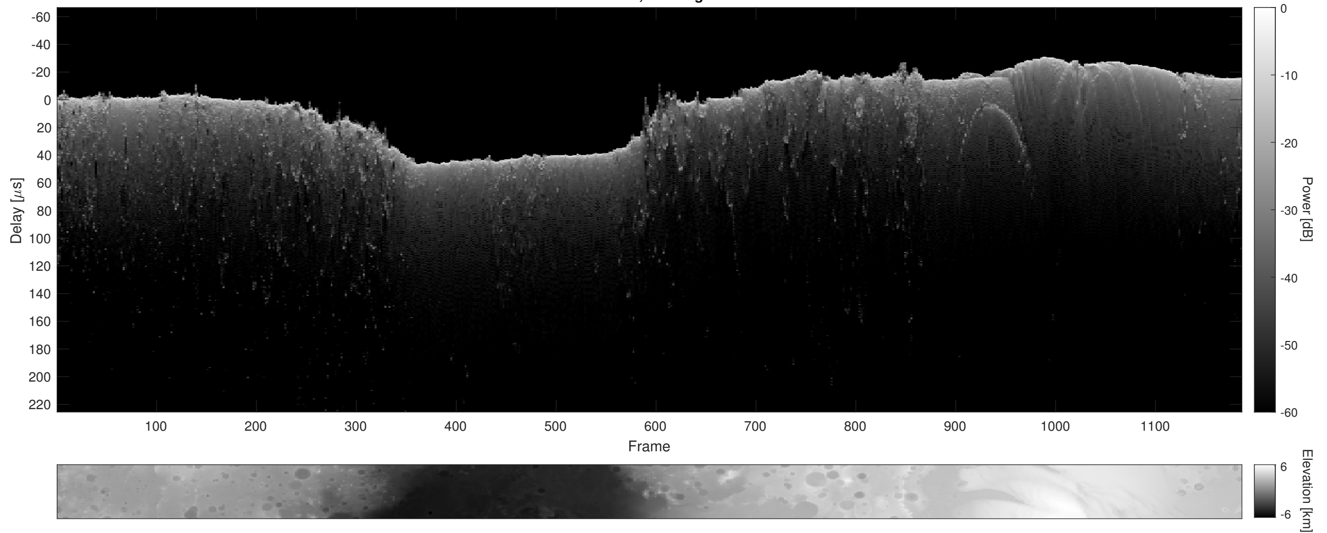
Orbit 8952, Cluttergram
