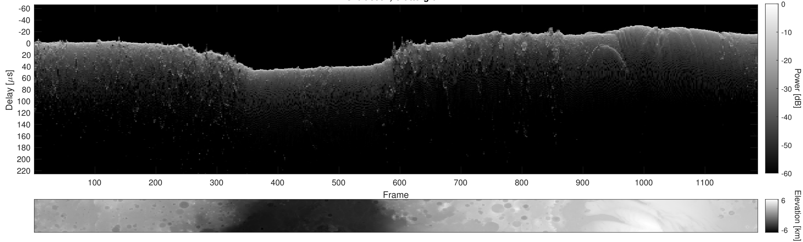
Orbit 8952, Cluttergram
