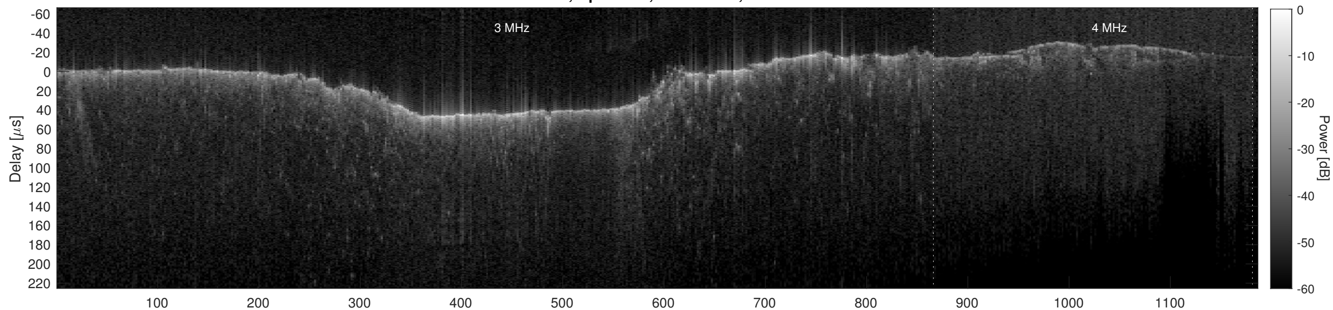
Orbit 8952, Cluttergram
