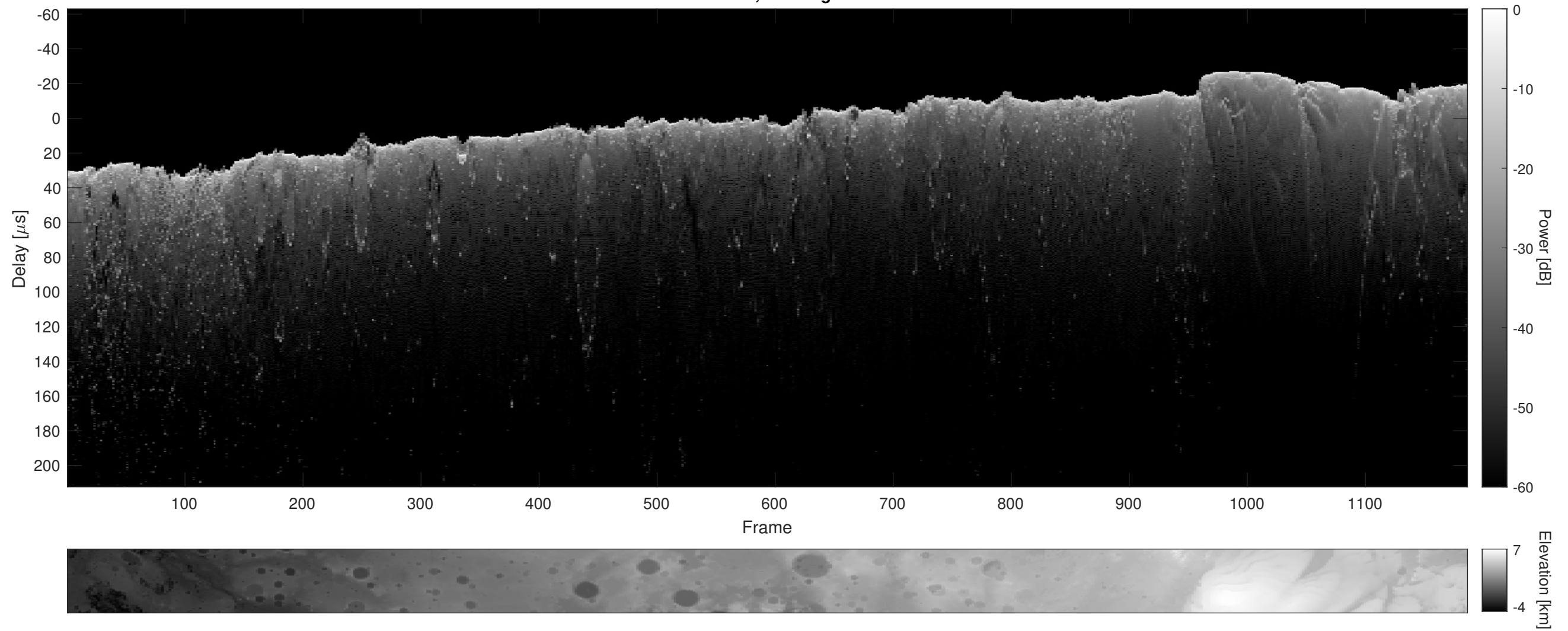
Orbit 8953, Cluttergram
