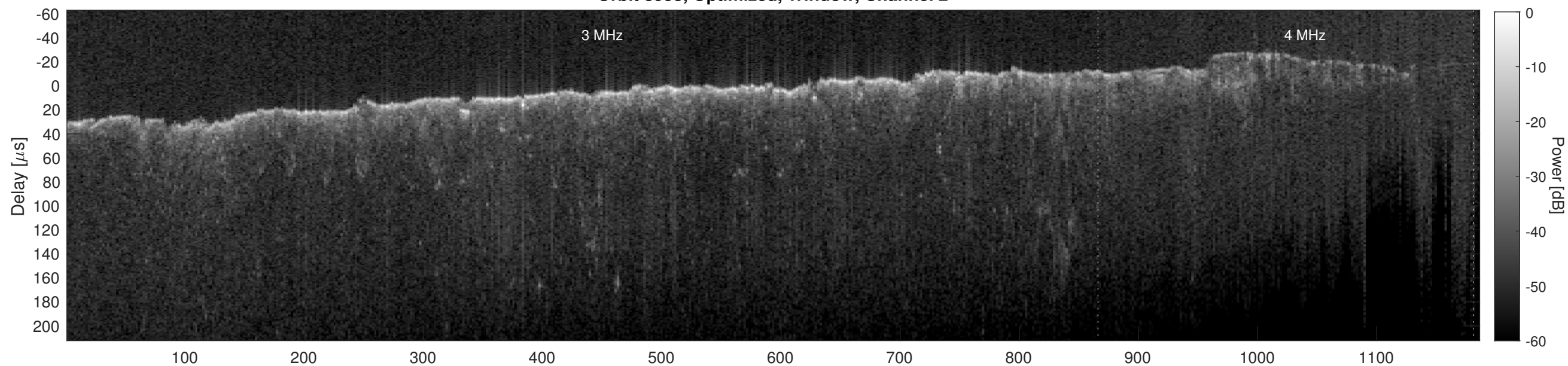
Orbit 8953, Cluttergram
