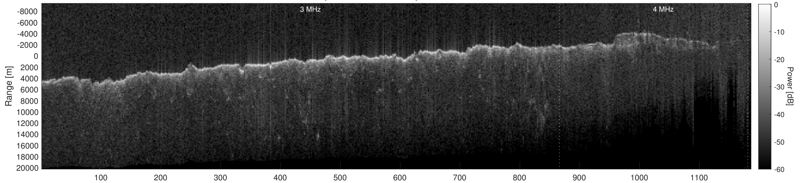
Orbit 8953, Depth-Corrected Cluttergram
