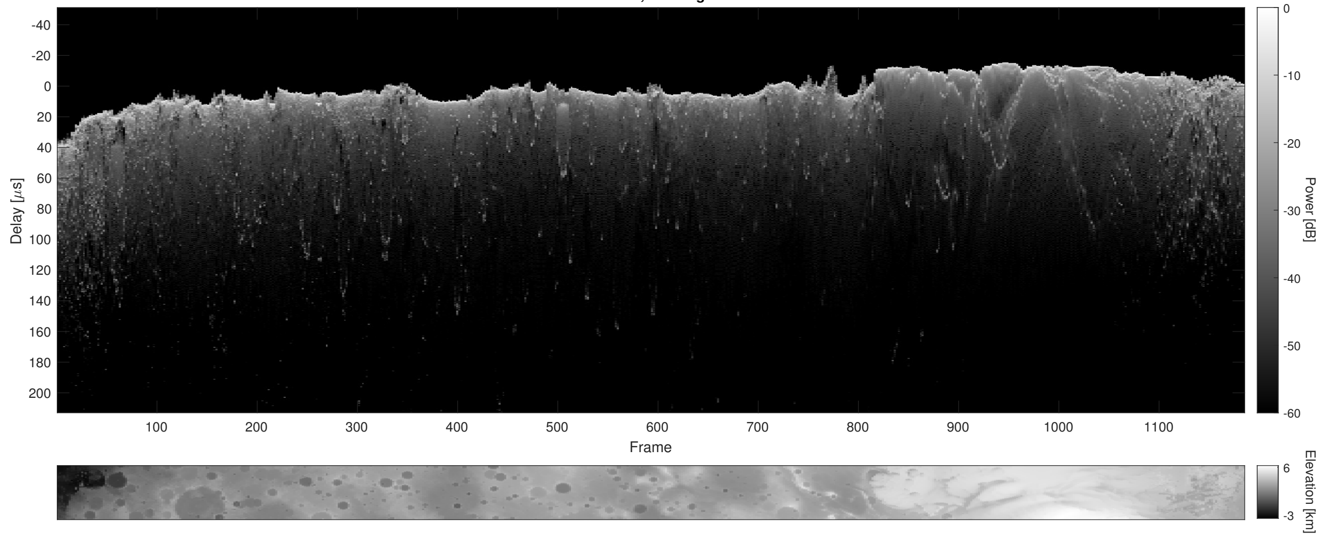
Orbit 8955, Cluttergram
