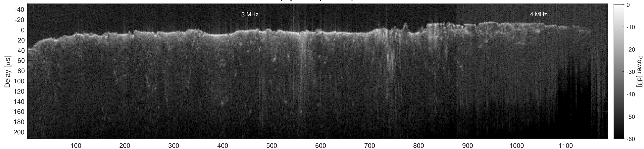
Orbit 8955, Cluttergram
