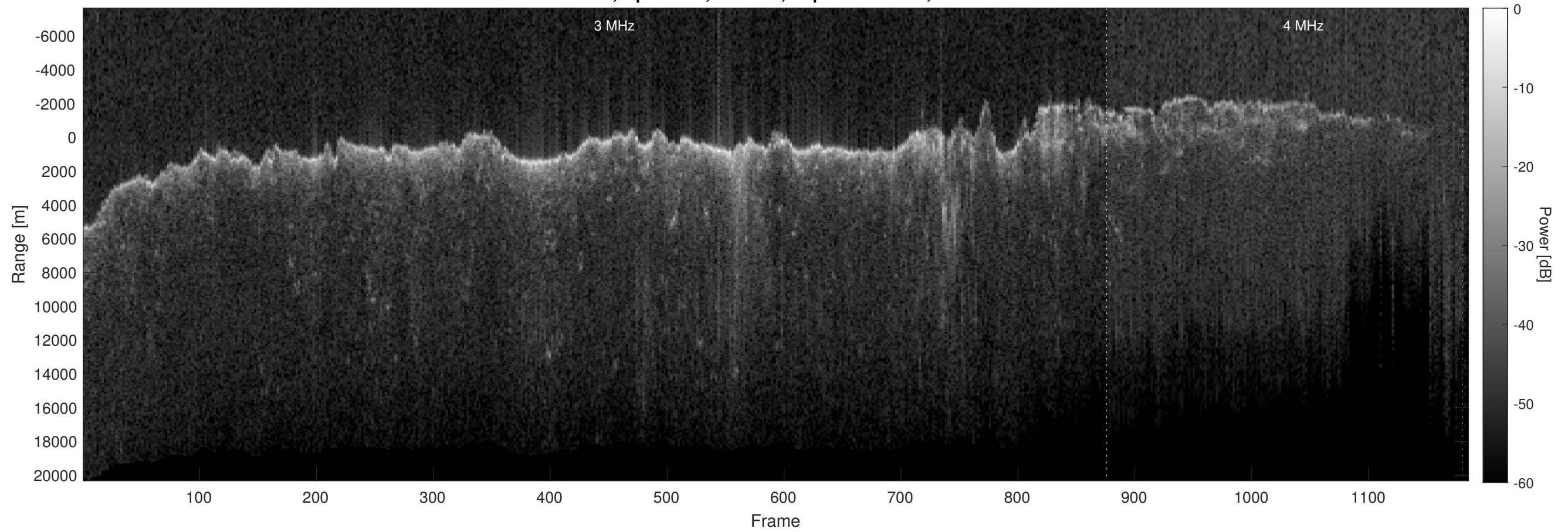
Orbit 8955, Optimized, Window, Depth-Corrected, Channel 2
